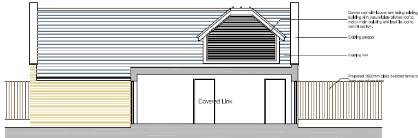
SOUTH FACING SECTIONAL ELEVATION
